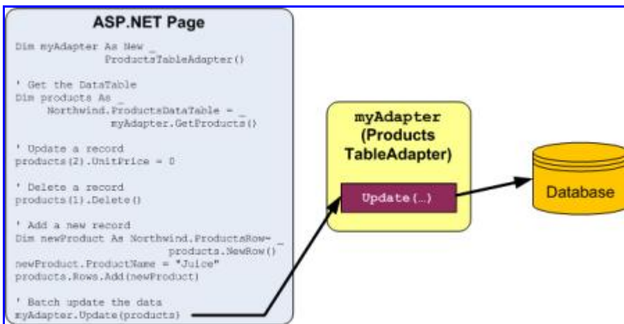
Figure 22: All Changes are Synchronized with the Database When the Update Method is Invoked
